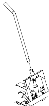
Figure 8: Handle assembly.
