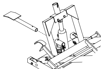
Figure 7: Foot Pedal assembly.
