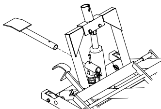
Figure 7: Foot Pedal assembly.
