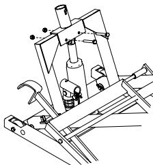
Figure 6: Handle Yoke assembly.
