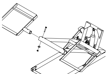
Figure 5: Fixation du support de roue
