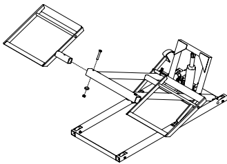
Figure 5: Wheel Basket attachment.
