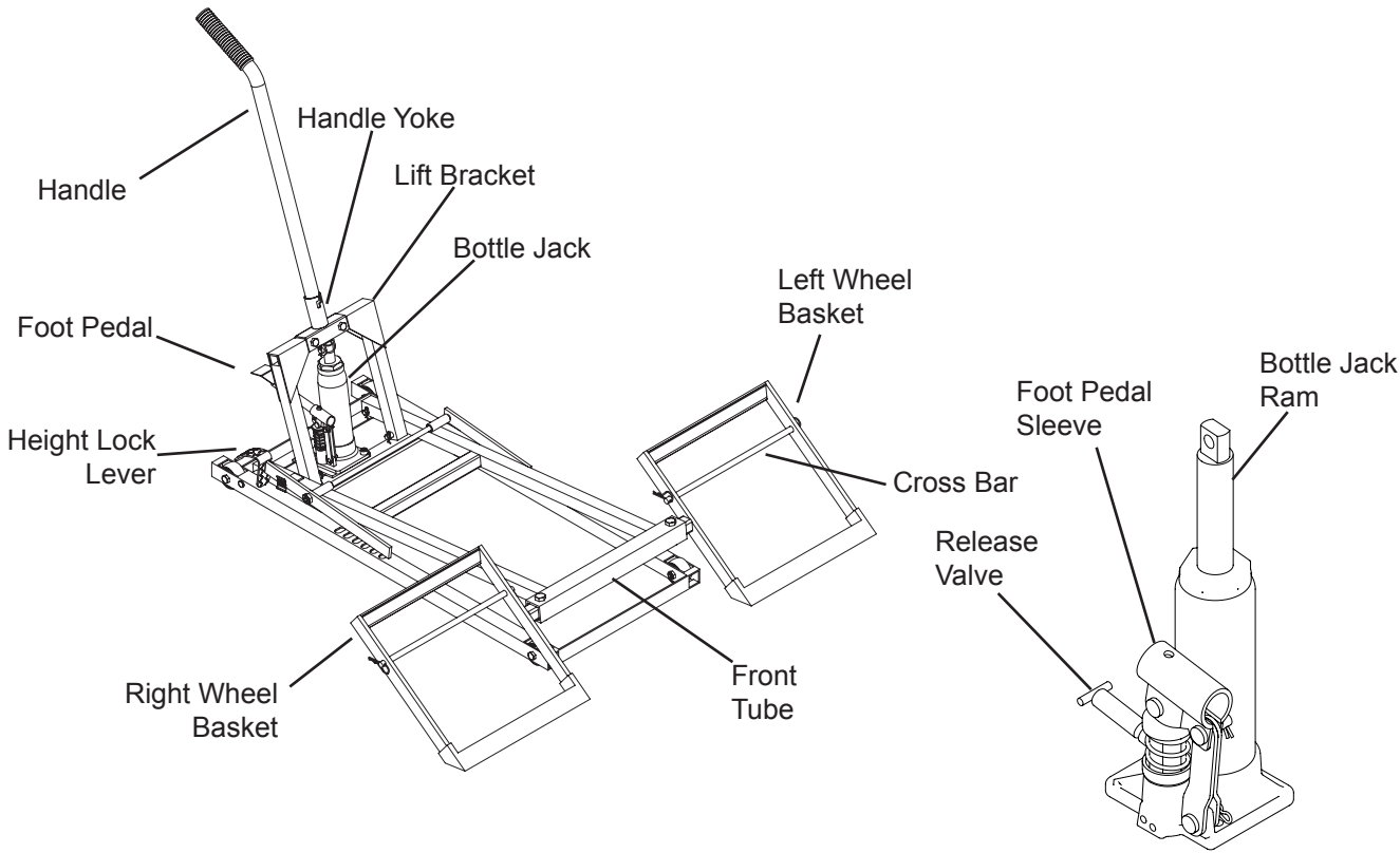
Figure 1: Lawn Mower Lift nomenclature.
