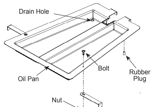
Figure 1 - Oil Drip Pan Illustration.
