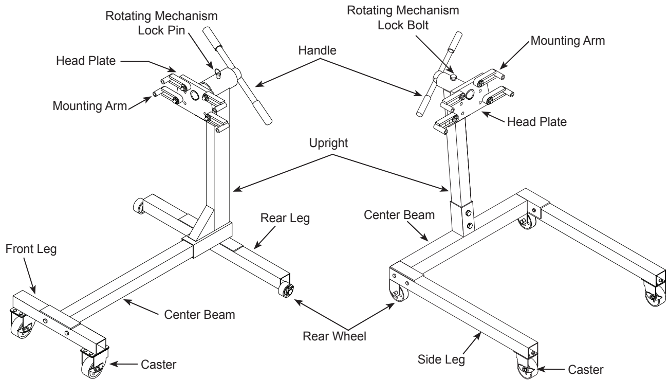
Figure 1 - Model 30750 Components
