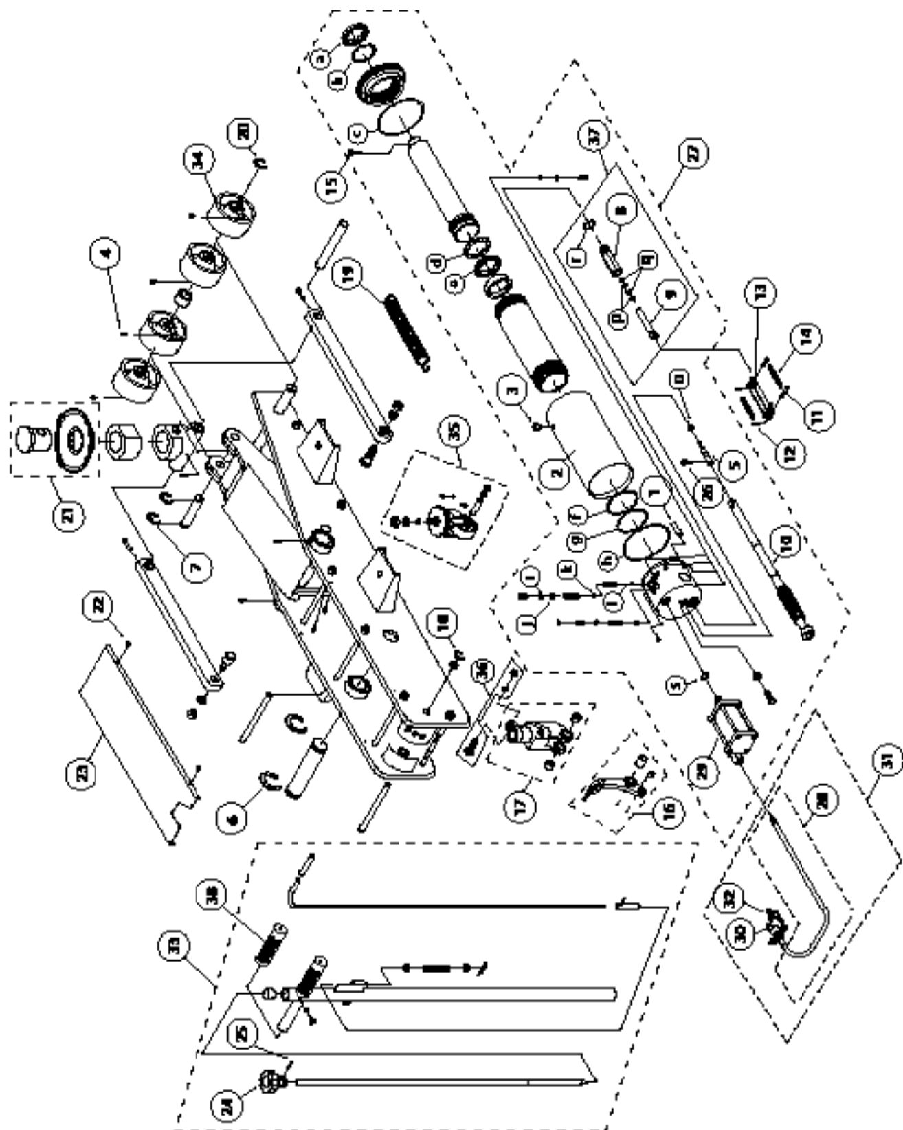
Figure 3 - Replacement Parts Illustration for Model 22203
